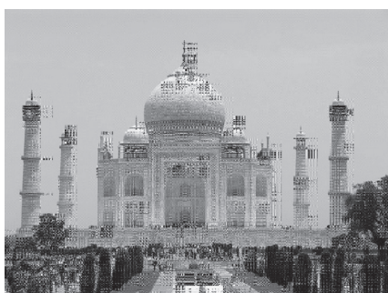
(e) Approximation 28 ( I_{28} ).
