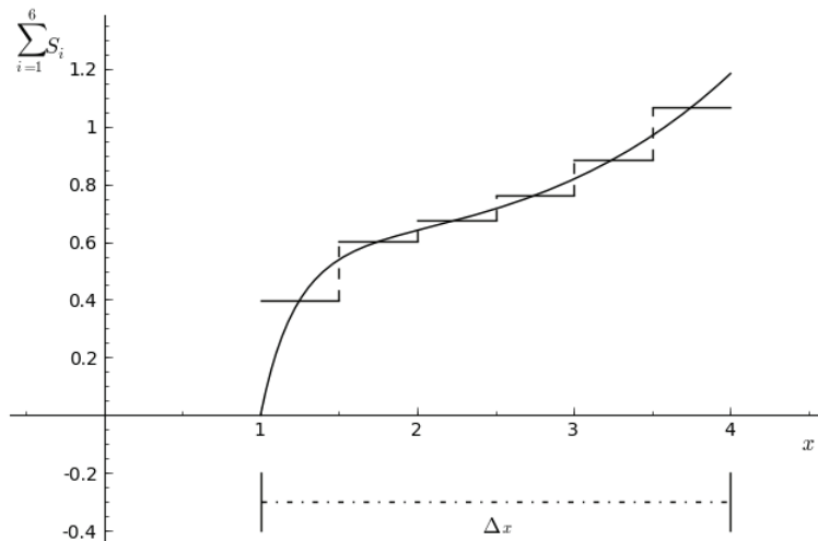
Figure 4: Approximation to f(x) , specified in (1) by \sum_{i=1}^6 S_i ; f(x) is indicated by a solid line.
