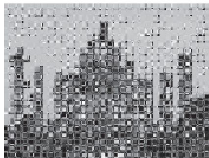
(b) Approximation 16 ( I_{16} ).
