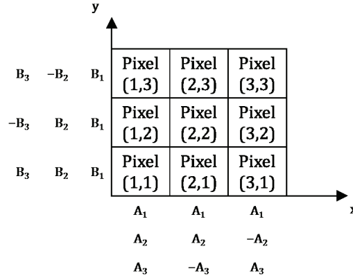
Figure 8: How to apply the SWM to the analysis of the image represented here, made up of 9 pixels.
