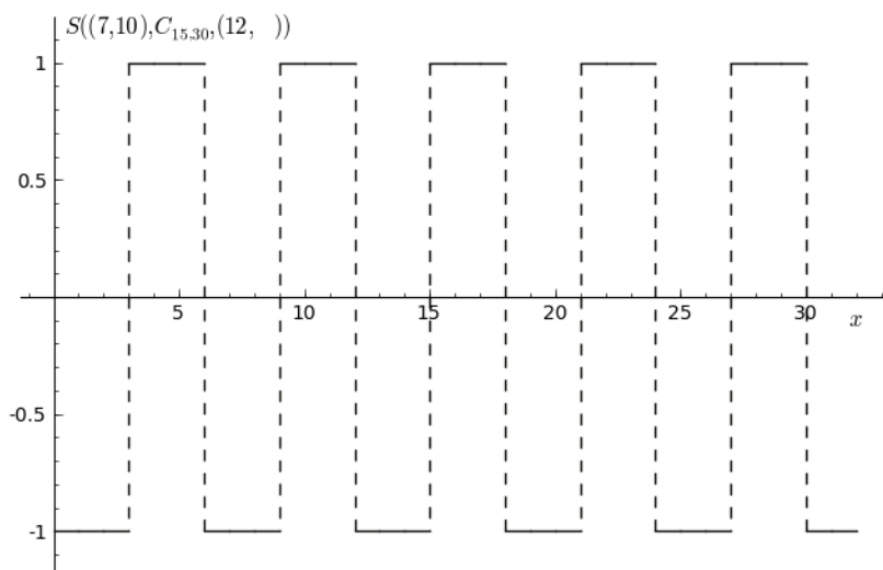
(b) S((7, 10), C_{15,30}, (12, \quad)) .
