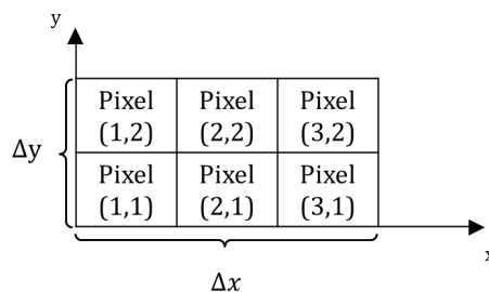
Figure 6: An image made up of 6 pixels.
