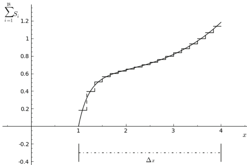
Figure 5: Approximation to f(x) specified in (1) by \sum_{i=1}^{18} S_i ; f(x) is indicated by a solid line.
