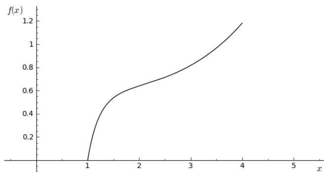
Figure 1: f(x) = \frac{\ln x \cdot e^x}{x^3} , 1 \leq x \leq 4 .
