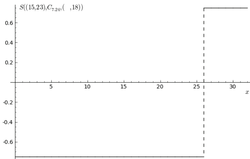
(a) [S((15, 23), C_{7,24}, ( \quad, 18)) .
