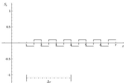
(f) S_6(x) .
