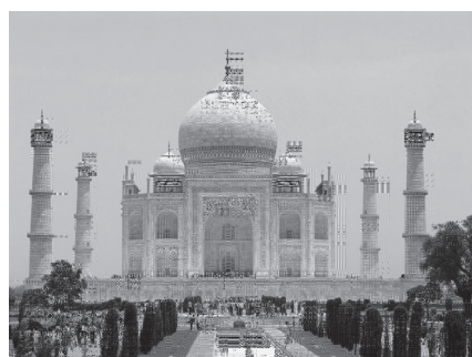
(f) Approximation 29 ( I_{29} ).
