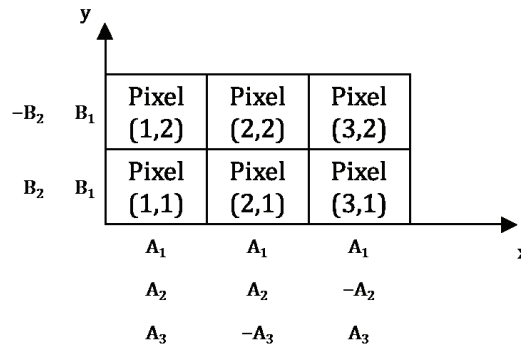
Figure 7: How to apply the SWM to the analysis of the image corresponding to figure 6.
