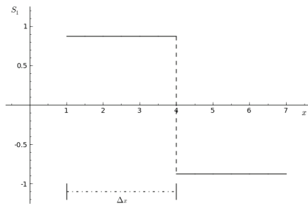
(a) S_1(x) .
