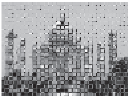
(a) Approximation 12 ( I_{12} ).
