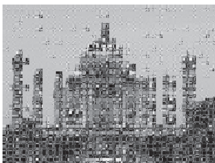
(c) Approximation 20 ( I_{20} ).
