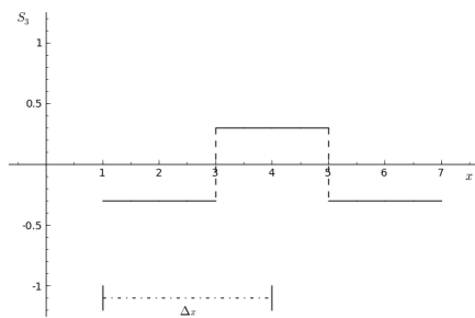
(c) S_3(x) .
