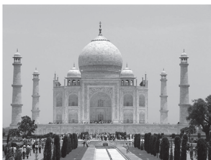
(i) Approximation 32 ( I_{32} ).
