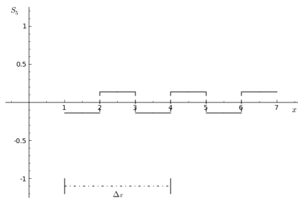
(e) S_5(x) .
